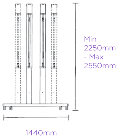
UltraTwin Freespan
